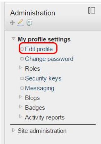
Figure 2: Administration panel
